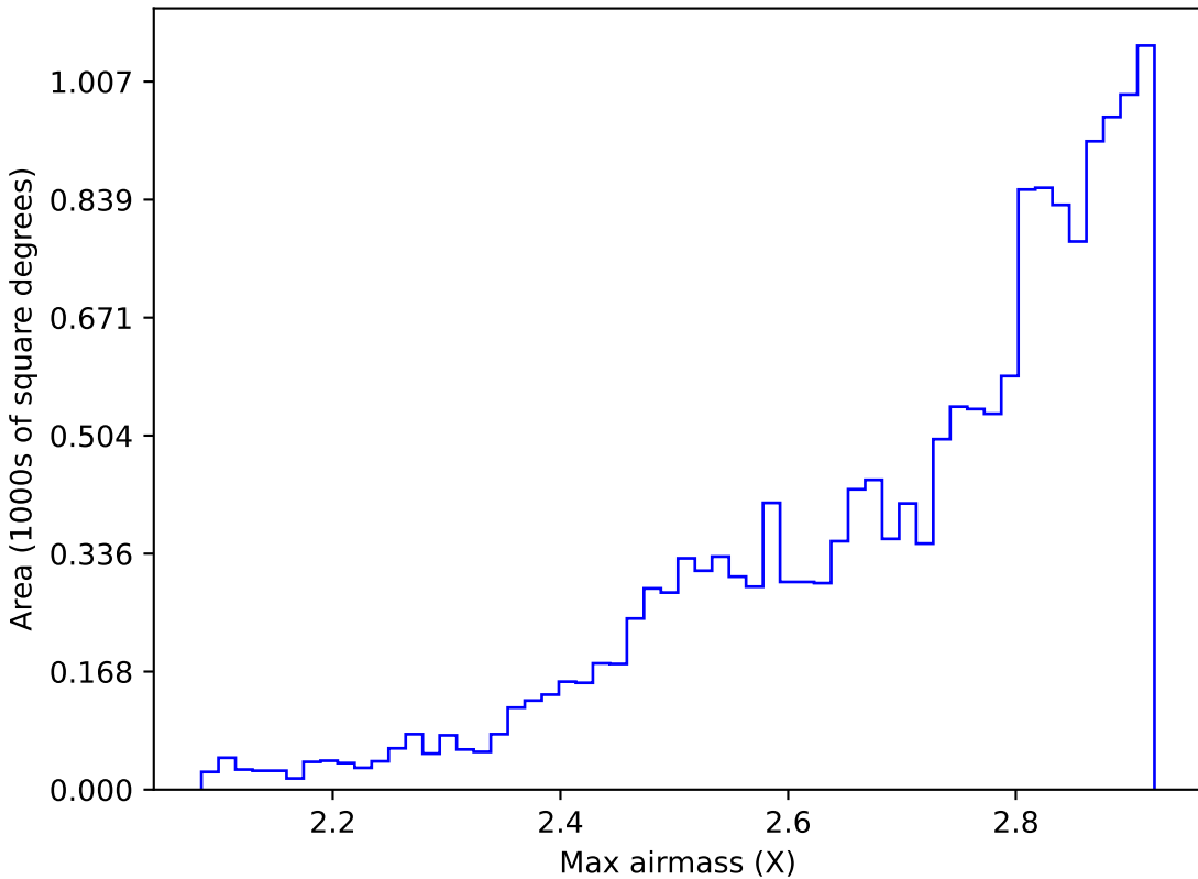
extra_ss_neo2_v3.4_10yrs WFD all bands: Max airmass
