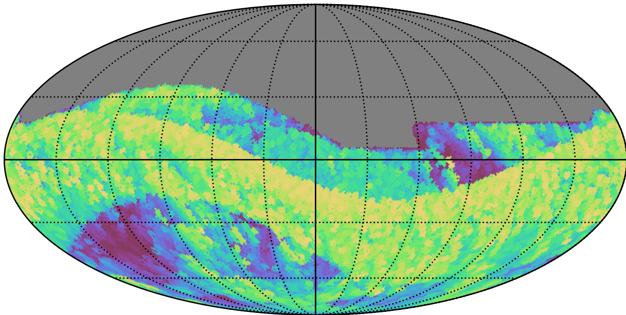
extra_ss_neo2_v3.4_10yrs All sky z band: Max airmass
