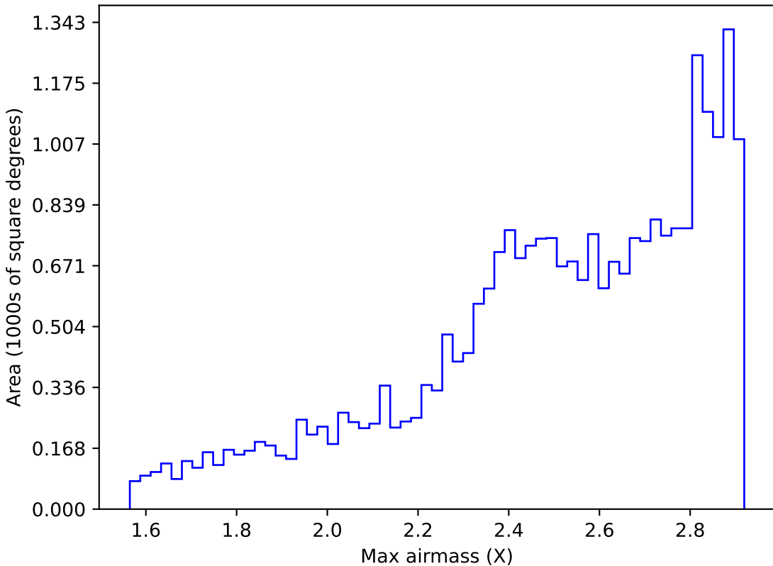
extra_ss_neo2_v3.4_10yrs All sky z band: Max airmass
