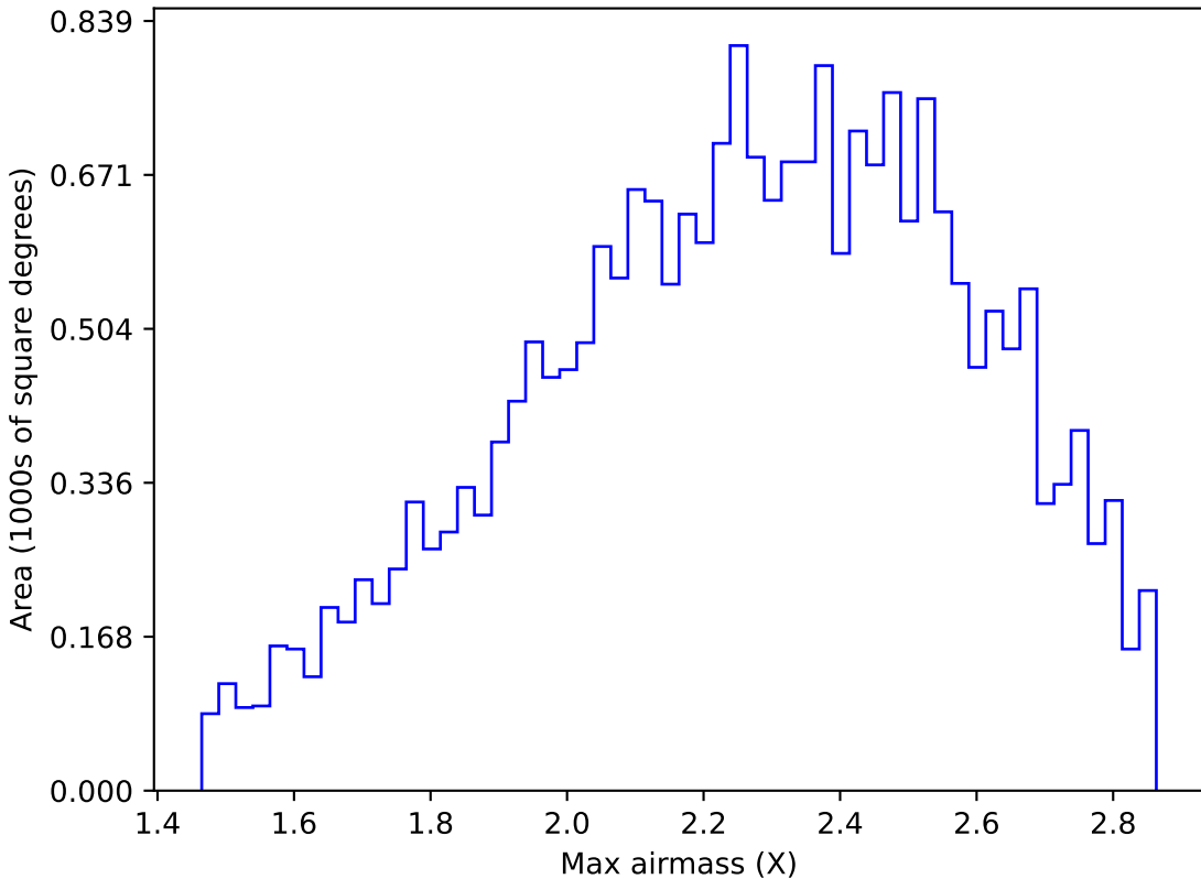
extra_ss_neo2_v3.4_10yrs All sky y band: Max airmass
