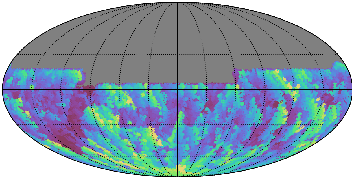
extra_ss_neo2_v3.4_10yrs All sky u band: Max airmass
