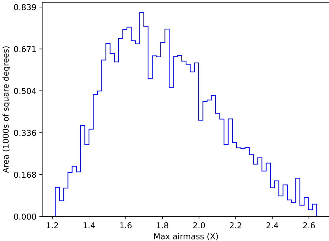
extra_ss_neo2_v3.4_10yrs All sky u band: Max airmass
