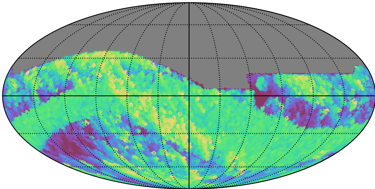
extra_ss_neo2_v3.4_10yrs All sky r band: Max airmass
