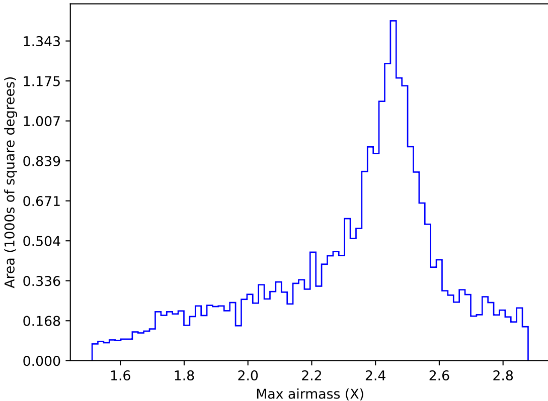
extra_ss_neo2_v3.4_10yrs All sky r band: Max airmass
