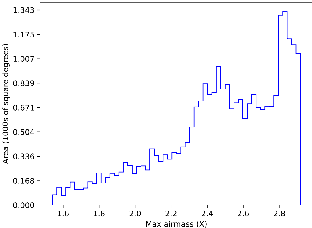
extra_ss_neo2_v3.4_10yrs All sky i band: Max airmass
