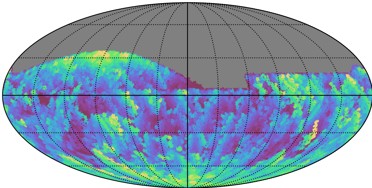
extra_ss_neo2_v3.4_10yrs All sky g band: Max airmass
