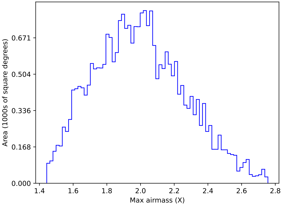
extra_ss_neo2_v3.4_10yrs All sky g band: Max airmass
