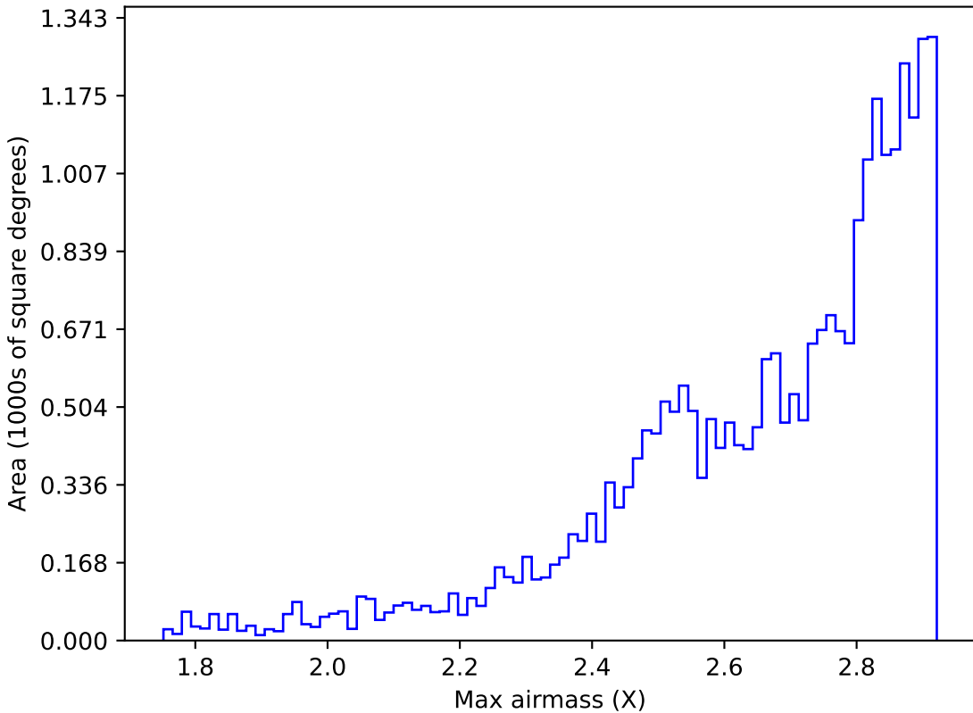
extra_ss_neo2_v3.4_10yrs All sky all bands: Max airmass
