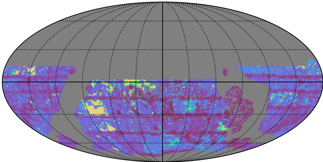
extra_ss_neo2_v3.4_10yrs WFD z band: Max Inter-Night Gap
