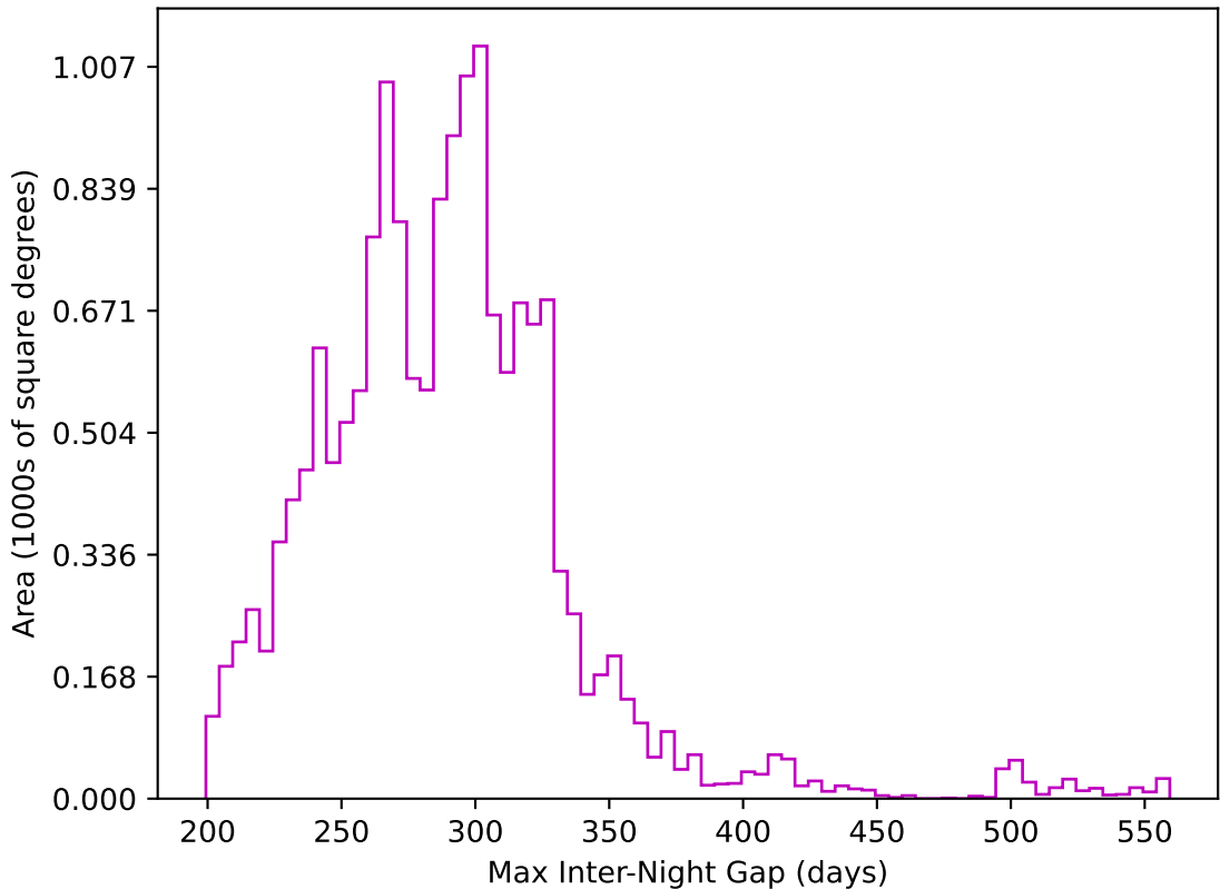
extra_ss_neo2_v3.4_10yrs WFD z band: Max Inter-Night Gap
