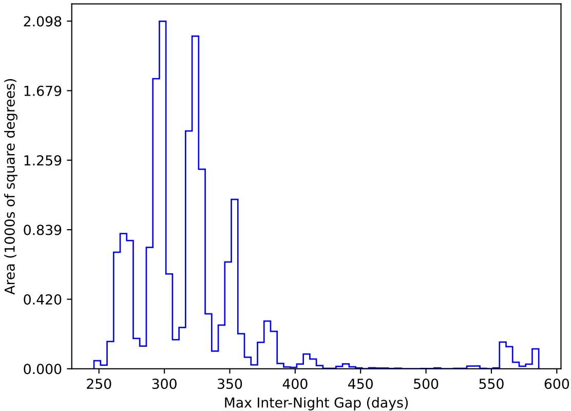
extra_ss_neo2_v3.4_10yrs WFD y band: Max Inter-Night Gap
