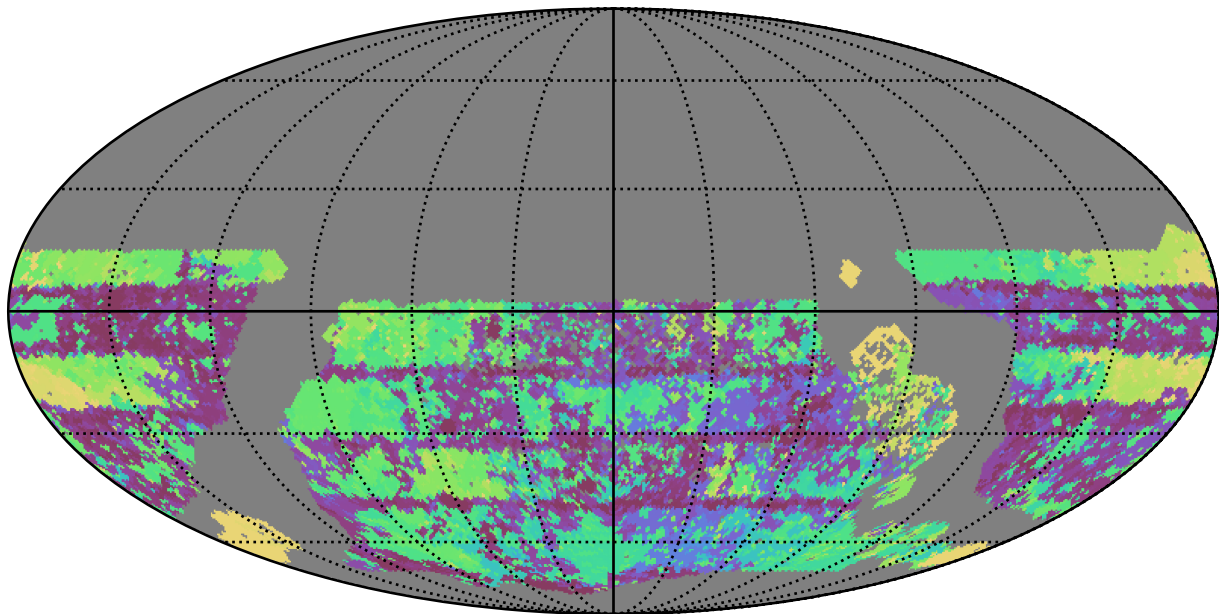
extra_ss_neo2_v3.4_10yrs WFD u band: Max Inter-Night Gap
