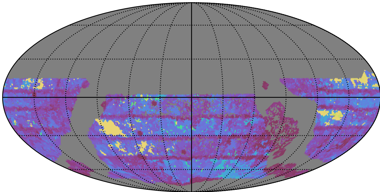
extra_ss_neo2_v3.4_10yrs WFD r band: Max Inter-Night Gap
