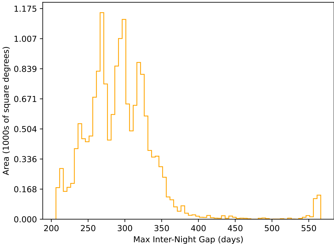
extra_ss_neo2_v3.4_10yrs WFD r band: Max Inter-Night Gap
