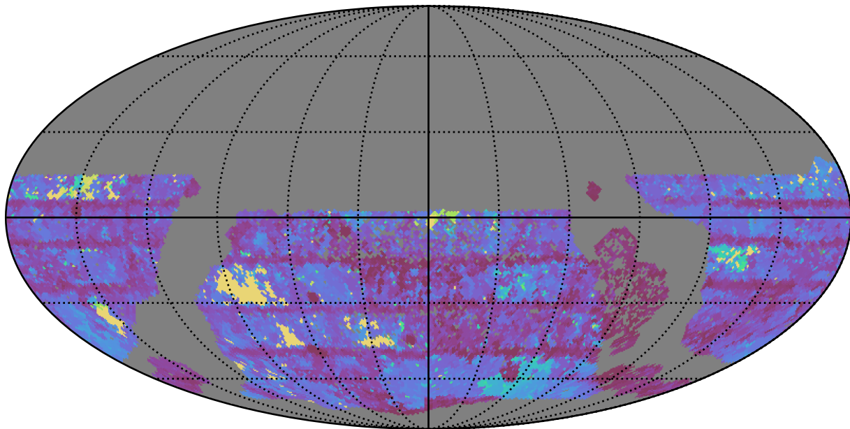
extra_ss_neo2_v3.4_10yrs WFD i band: Max Inter-Night Gap
