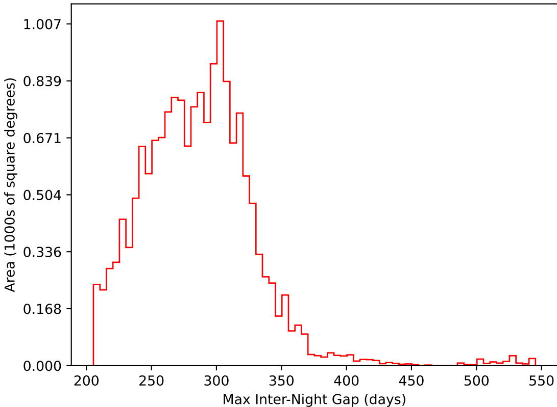
extra_ss_neo2_v3.4_10yrs WFD i band: Max Inter-Night Gap
