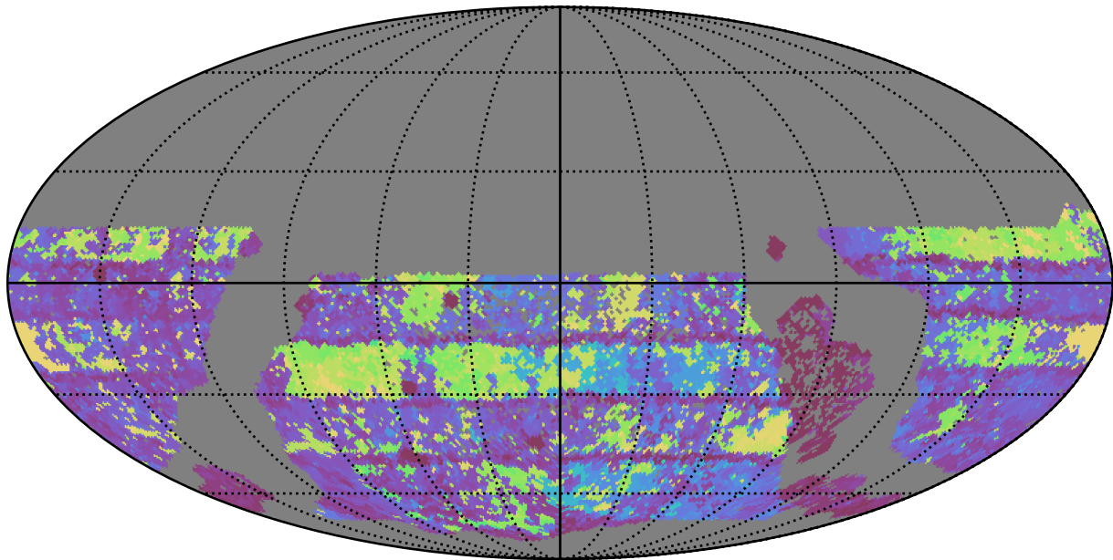
extra_ss_neo2_v3.4_10yrs WFD g band: Max Inter-Night Gap
