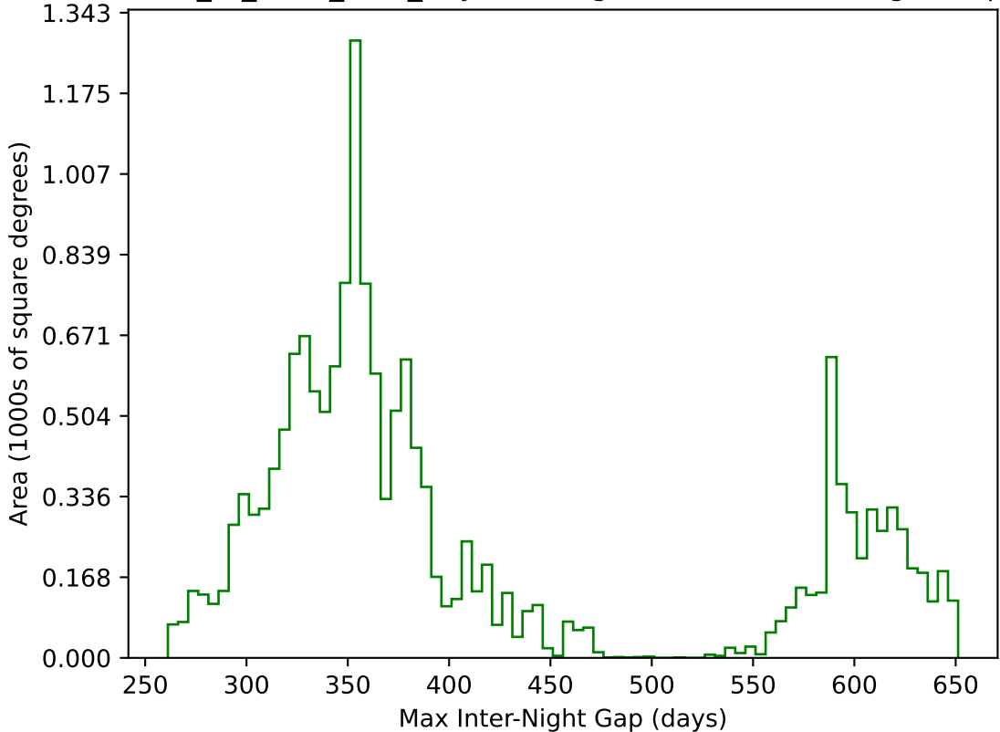
extra_ss_neo2_v3.4_10yrs WFD g band: Max Inter-Night Gap
