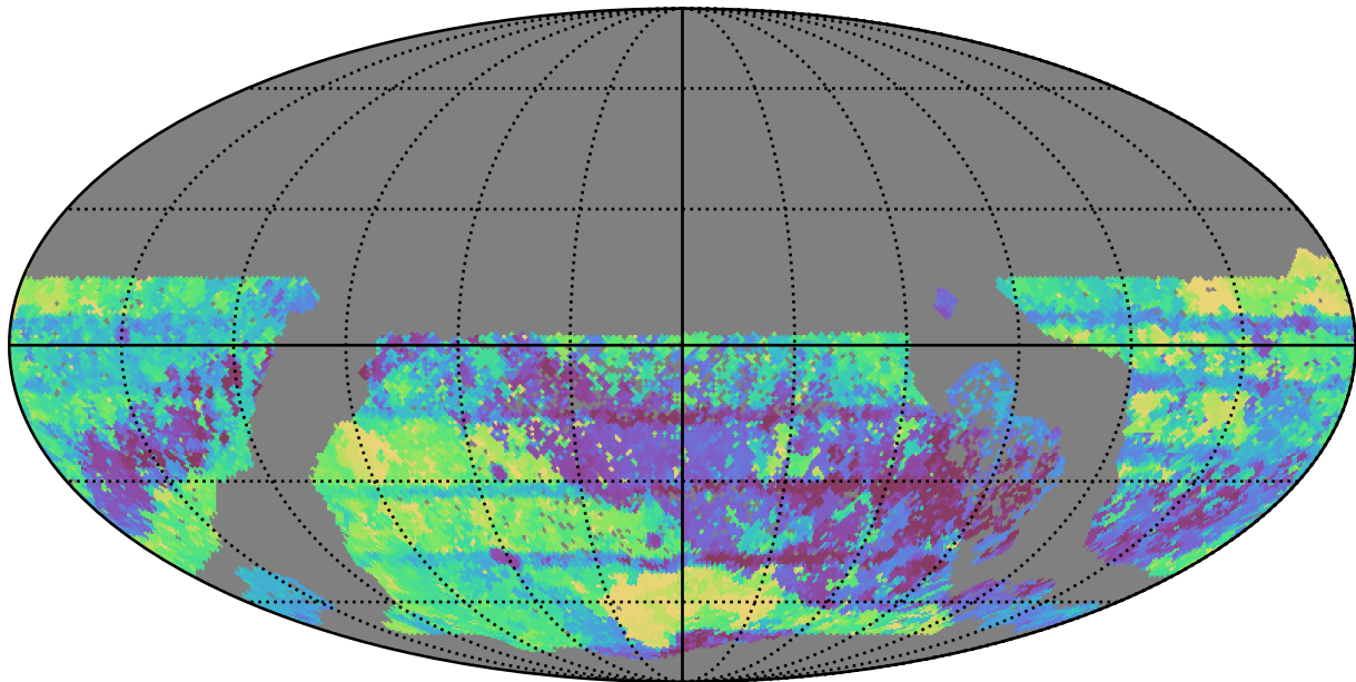
extra_ss_neo2_v3.4_10yrs WFD all bands: Max Inter-Night Gap
