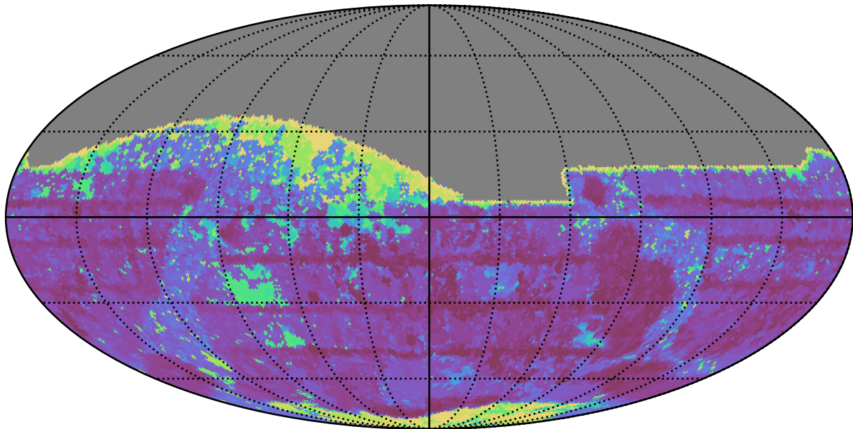
extra_ss_neo2_v3.4_10yrs All sky z band: Max Inter-Night Gap
