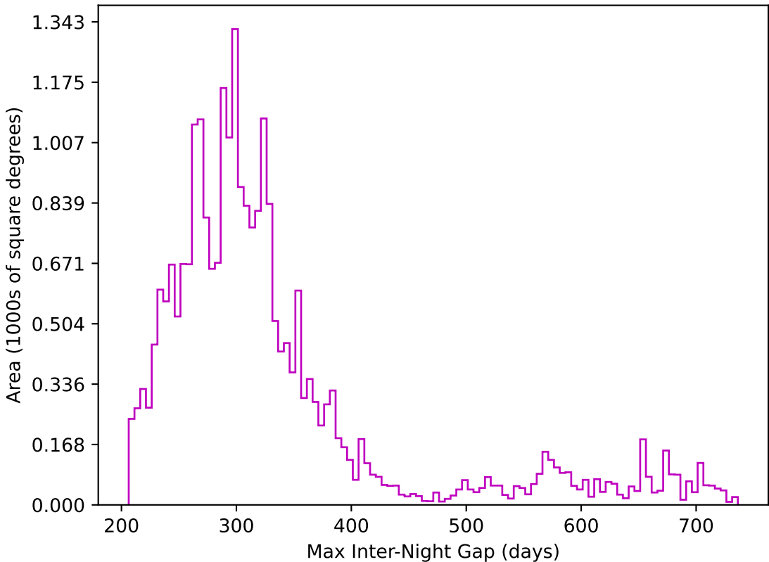
extra_ss_neo2_v3.4_10yrs All sky z band: Max Inter-Night Gap
