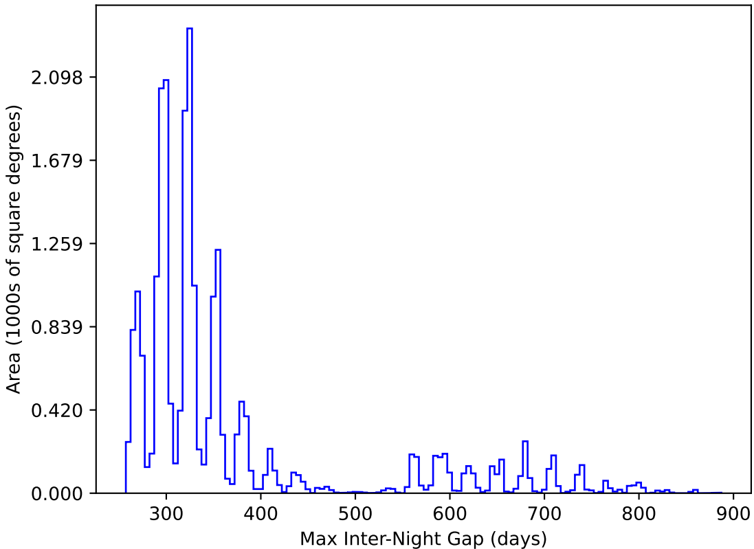
extra_ss_neo2_v3.4_10yrs All sky y band: Max Inter-Night Gap
