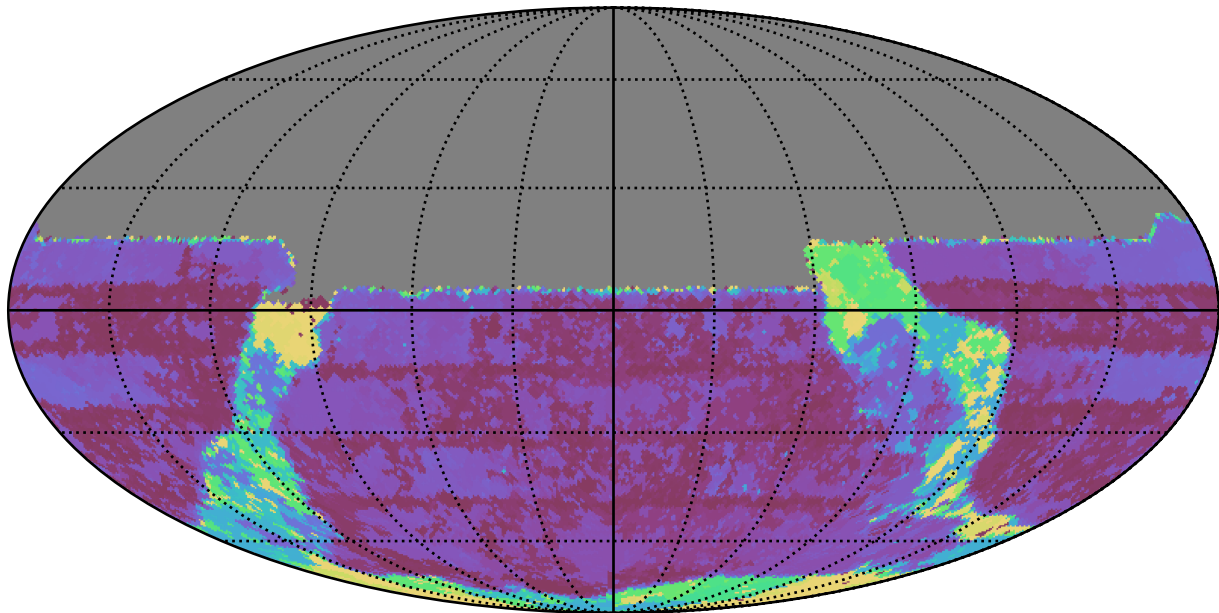
extra_ss_neo2_v3.4_10yrs All sky u band: Max Inter-Night Gap
