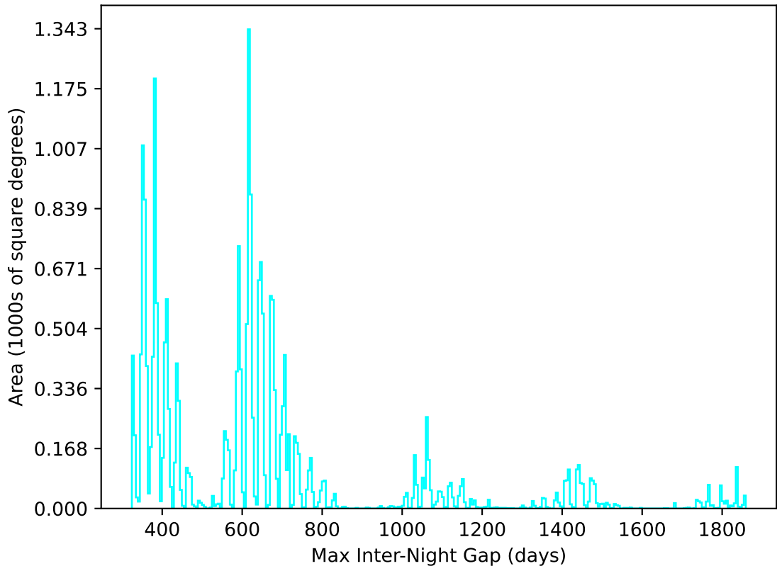
extra_ss_neo2_v3.4_10yrs All sky u band: Max Inter-Night Gap
