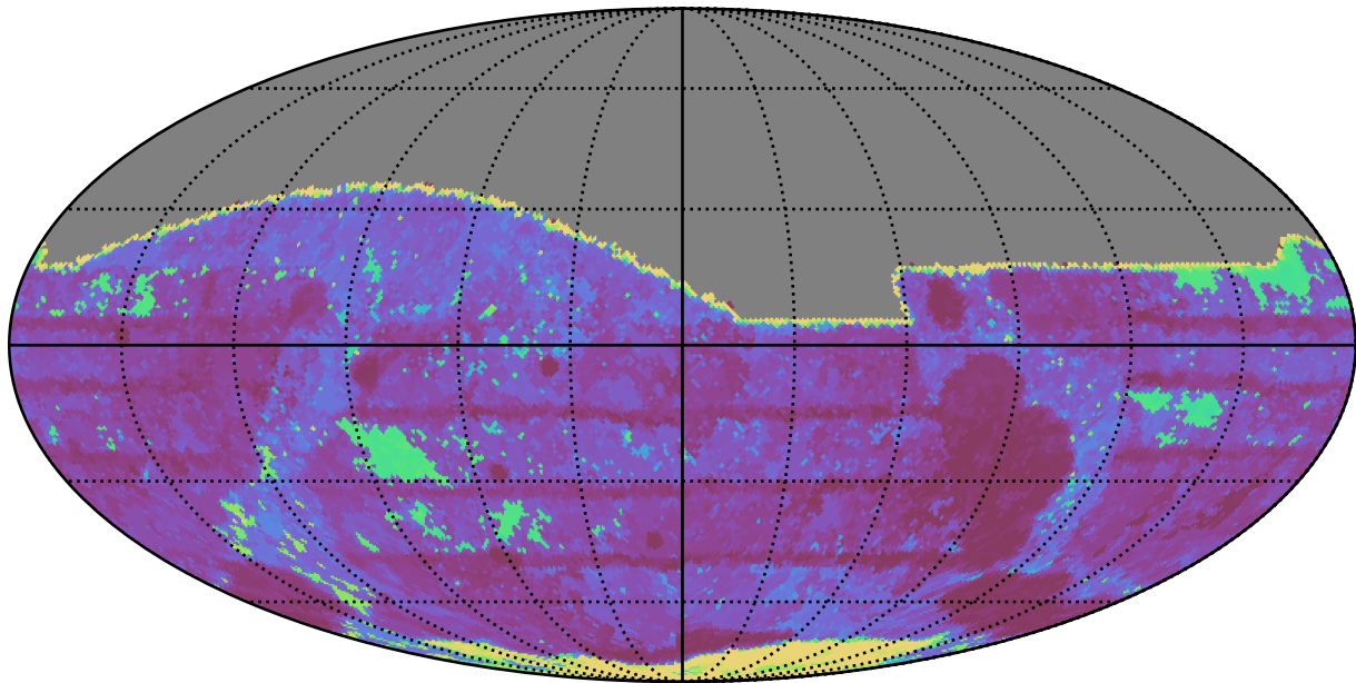
extra_ss_neo2_v3.4_10yrs All sky r band: Max Inter-Night Gap
