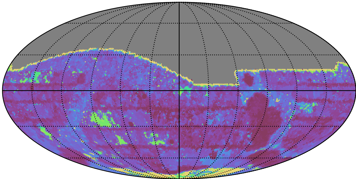
extra_ss_neo2_v3.4_10yrs All sky i band: Max Inter-Night Gap
