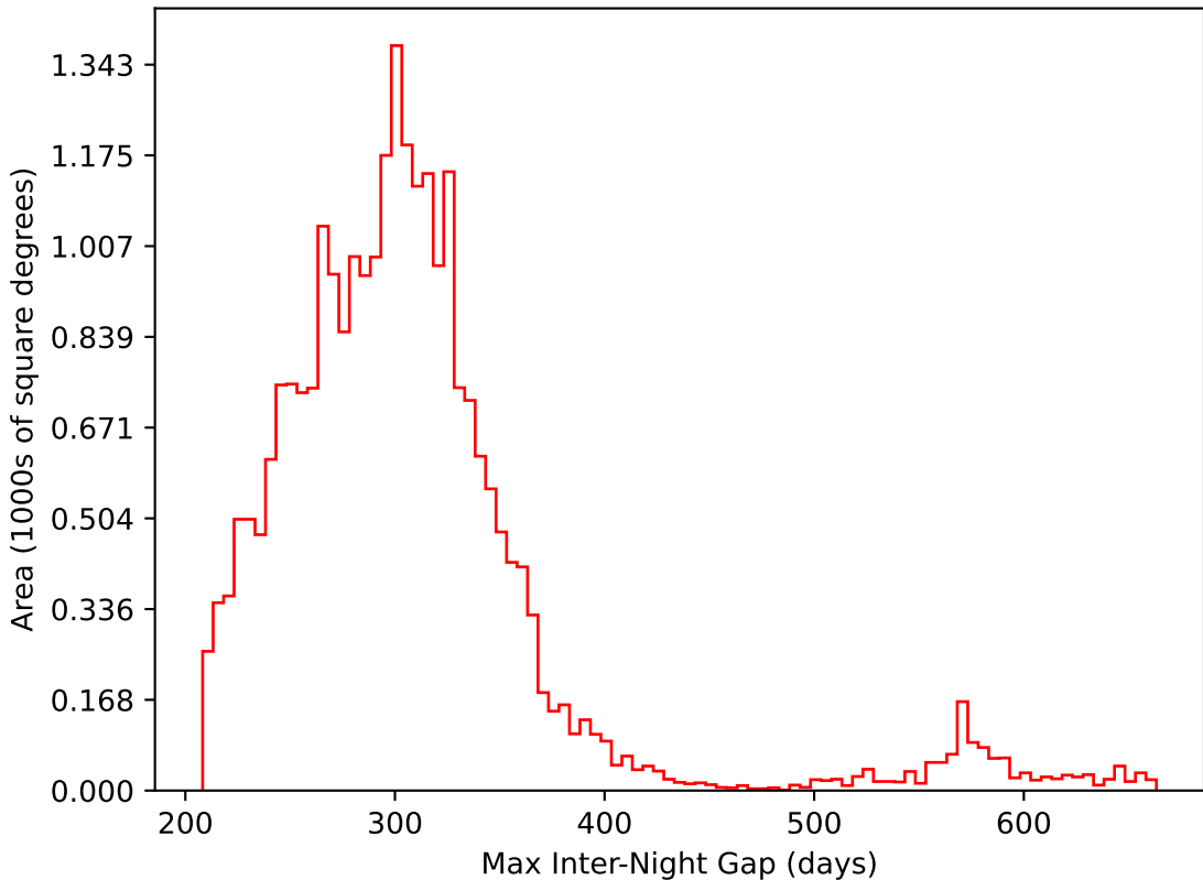
extra_ss_neo2_v3.4_10yrs All sky i band: Max Inter-Night Gap
