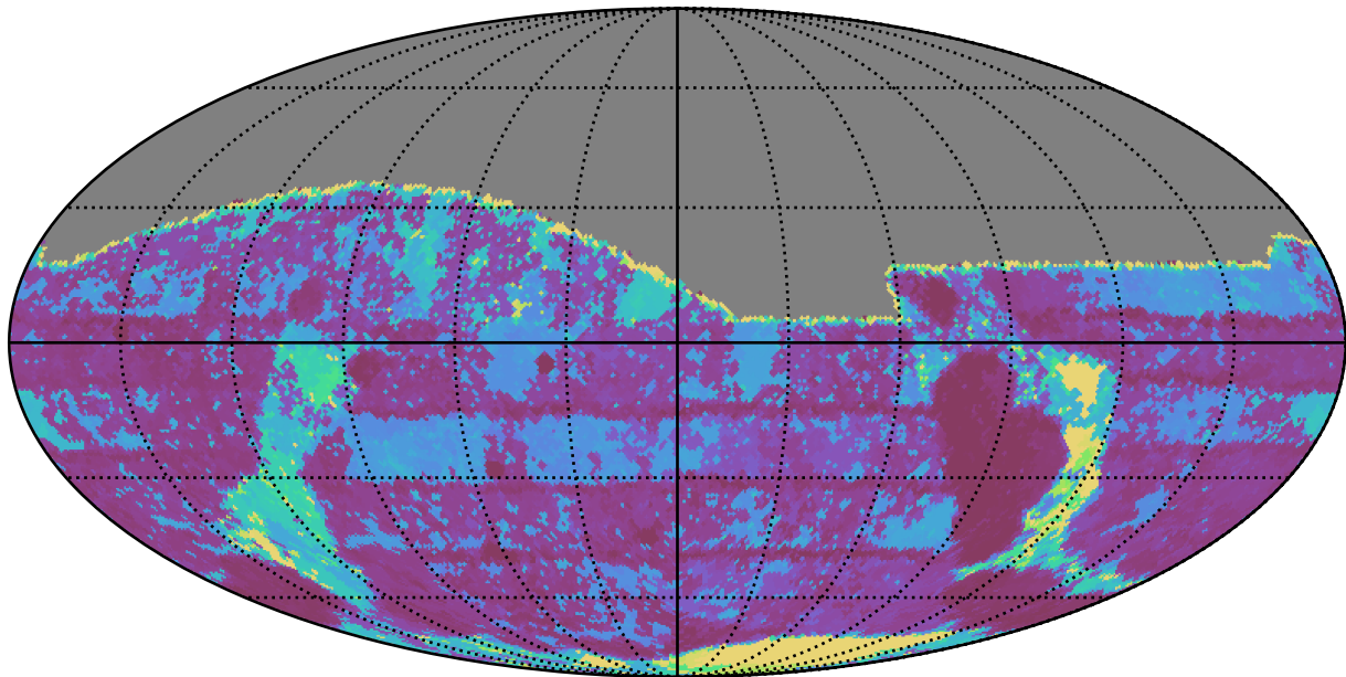
extra_ss_neo2_v3.4_10yrs All sky g band: Max Inter-Night Gap
