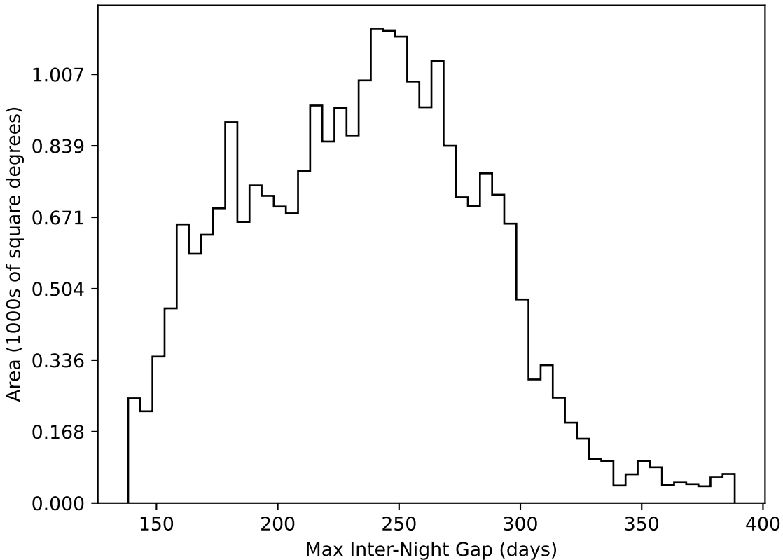
extra_ss_neo2_v3.4_10yrs All sky all bands: Max Inter-Night Gap
