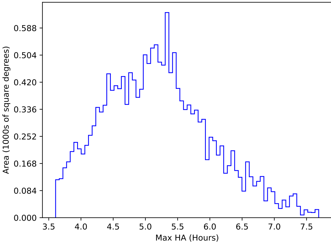
extra_ss_neo2_v3.4_10yrs WFD all bands: Max HA
