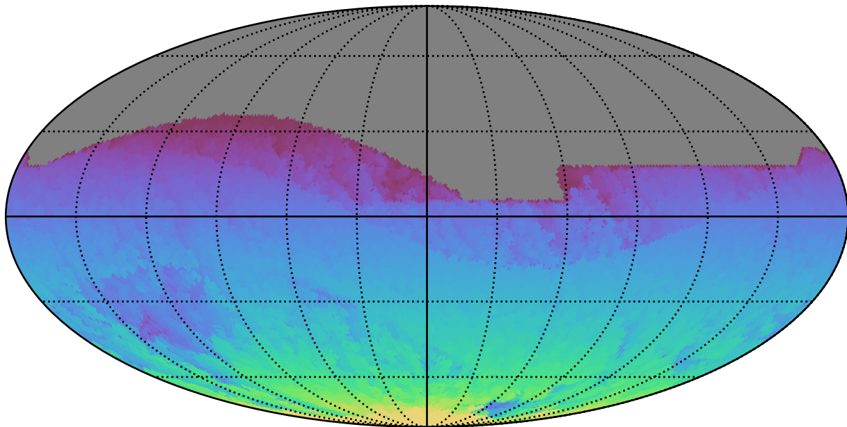
extra_ss_neo2_v3.4_10yrs All sky all bands: Max HA
