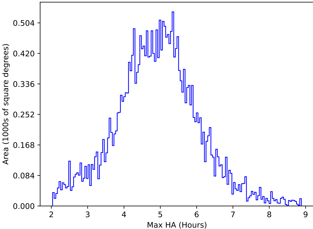
extra_ss_neo2_v3.4_10yrs All sky all bands: Max HA
