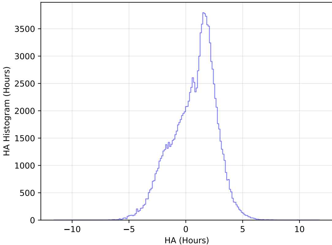
extra_ss_neo2_v3.4_10yrs WFD u band: HA Histogram
