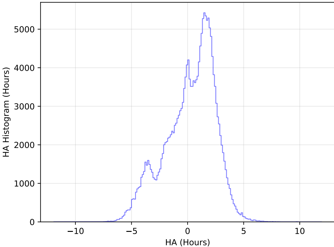
extra_ss_neo2_v3.4_10yrs WFD g band: HA Histogram
