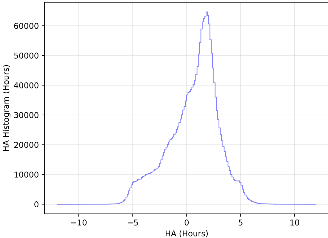
extra_ss_neo2_v3.4_10yrs WFD all bands: HA Histogram
