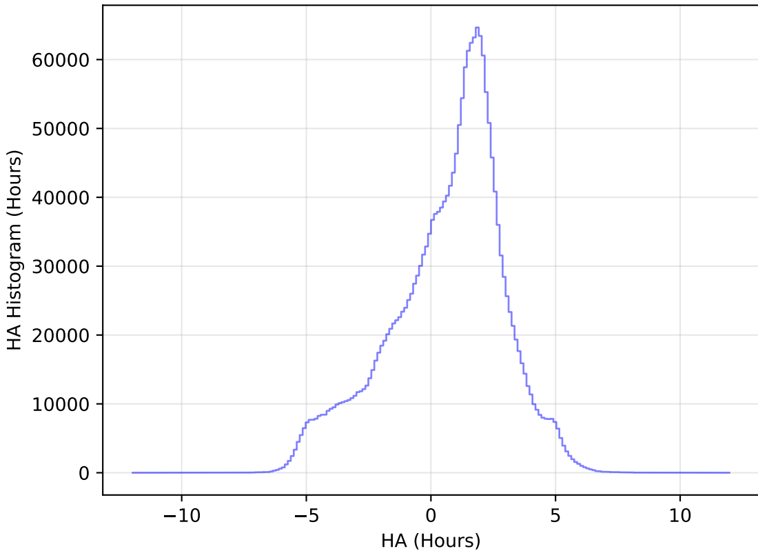
extra_ss_neo2_v3.4_10yrs All sky all bands: HA Histogram
