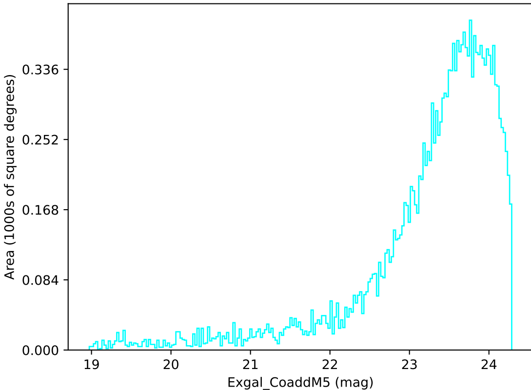
extra_ss_neo2_v3.4_10yrs Yr 3-4 u band: Exgal_CoaddM5
