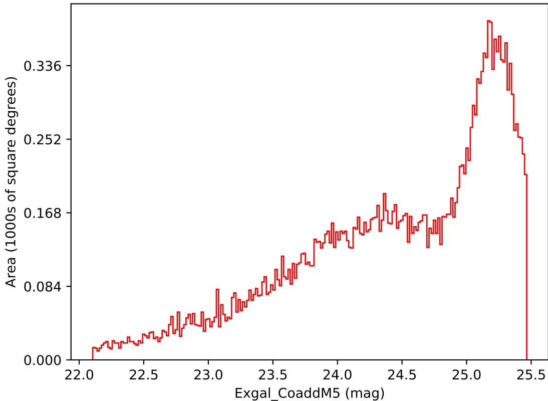
extra_ss_neo2_v3.4_10yrs Yr 3-4 i band: Exgal_CoaddM5
