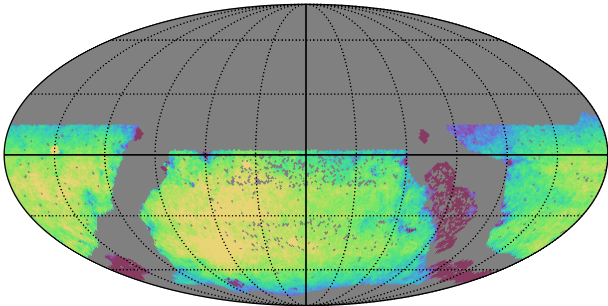
extra_ss_neo2_v3.4_10yrs WFD z band: Exgal_CoaddM5
