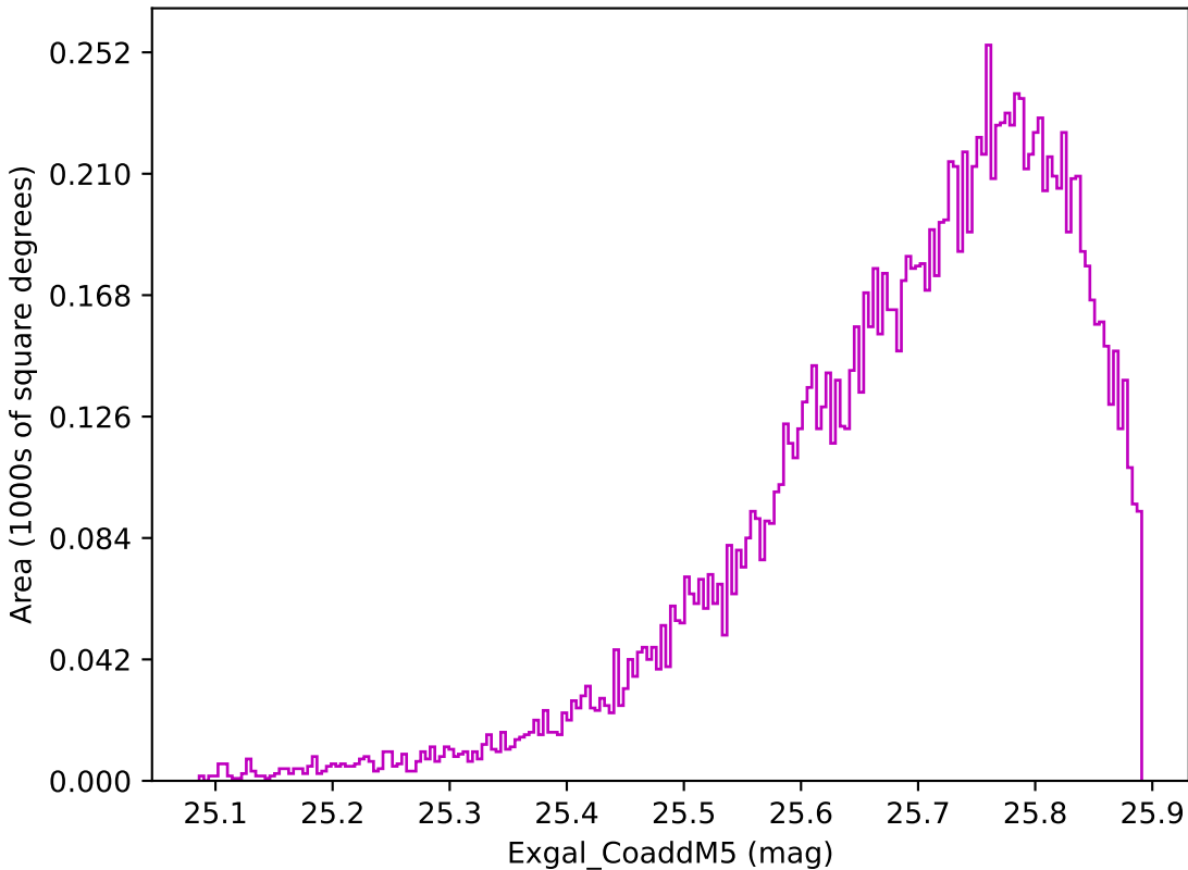
extra_ss_neo2_v3.4_10yrs WFD z band: Exgal_CoaddM5
