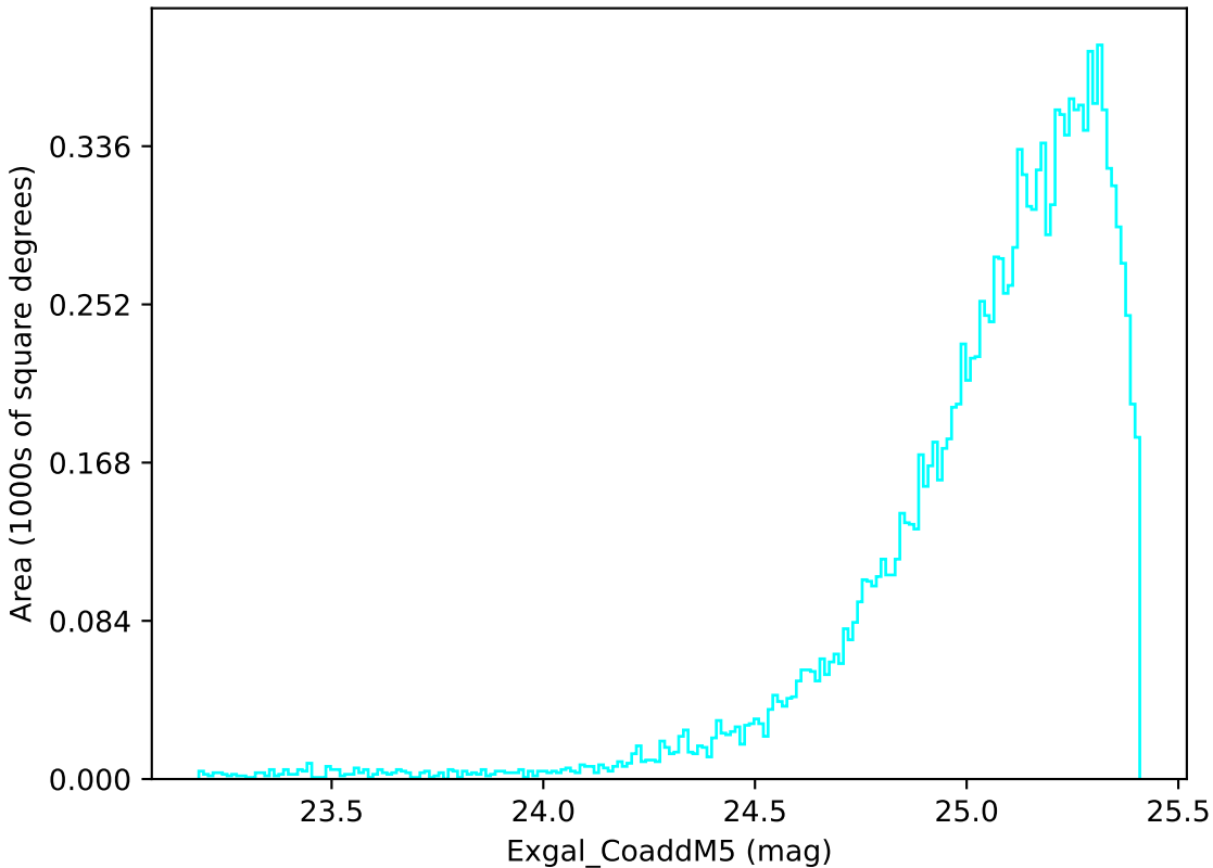
extra_ss_neo2_v3.4_10yrs WFD u band: Exgal_CoaddM5
