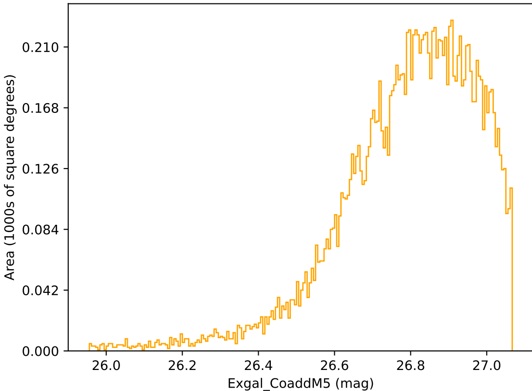
extra_ss_neo2_v3.4_10yrs WFD r band: Exgal_CoaddM5
