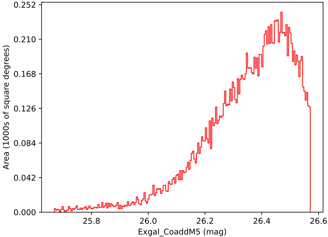
extra_ss_neo2_v3.4_10yrs WFD i band: Exgal_CoaddM5
