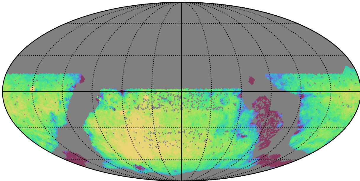
extra_ss_neo2_v3.4_10yrs WFD g band: Exgal_CoaddM5
