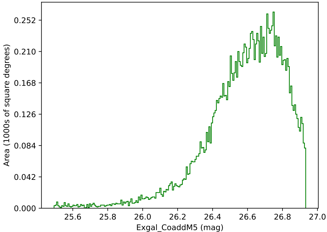
extra_ss_neo2_v3.4_10yrs WFD g band: Exgal_CoaddM5
