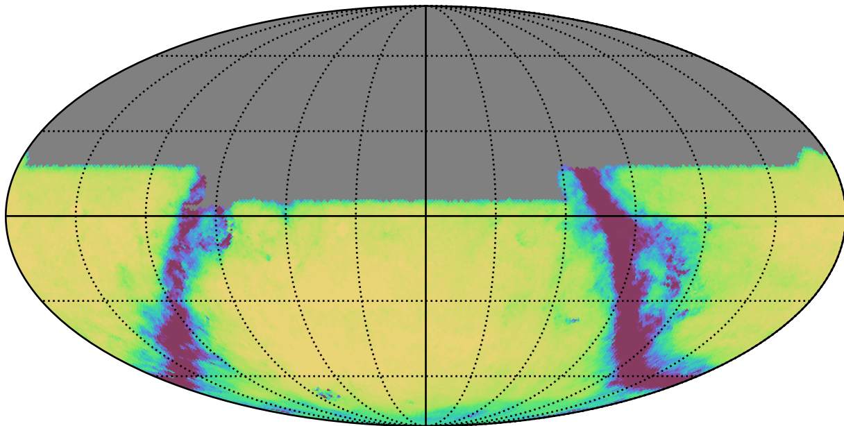
extra_ss_neo2_v3.4_10yrs All sky u band: Exgal_CoaddM5
